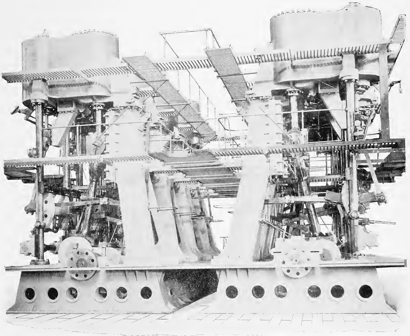
QUADRUPLE-EXPANSION ENGINES OF THE STEAMER NORTH WEST.
